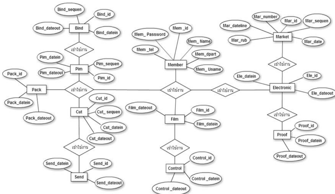
Fig. 2. ER diagram of the system
